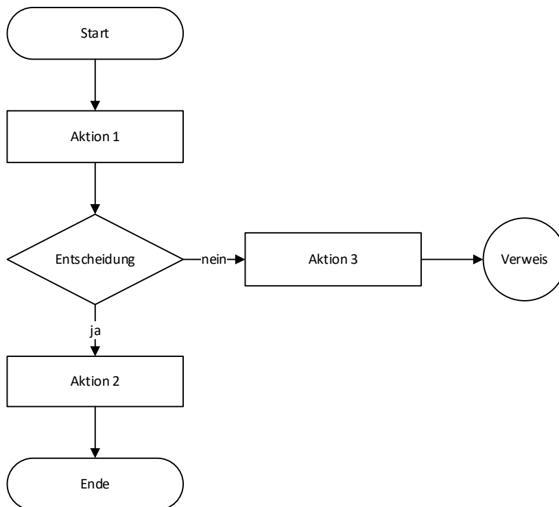
Abbildung 1: KPQM-Flowchart (Muster)
